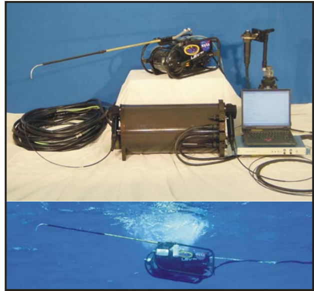
Figure 3. MOS ROV system components. The top panel shows the L_u and E_s input fibers and collectors, the ROV, and the ROV control system. The lower panel shows the input fiber for L_u , the ROV, and the optical/electrical umbilical that terminates on deck to MOS and the ROV control system.
